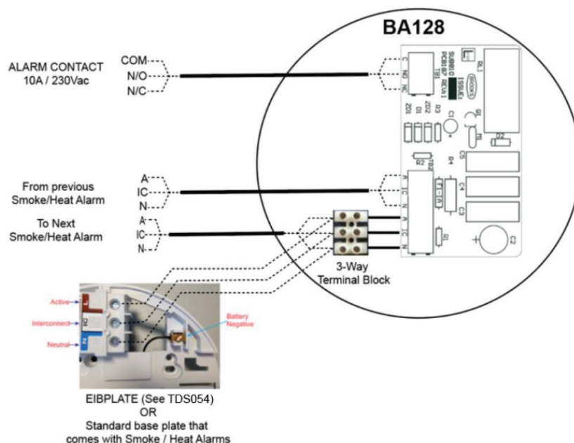
Figure 1 BA128 Wiring
