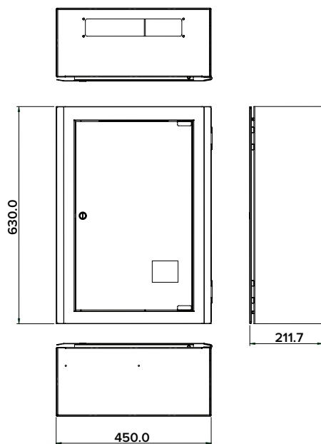
Standard Enclosure
