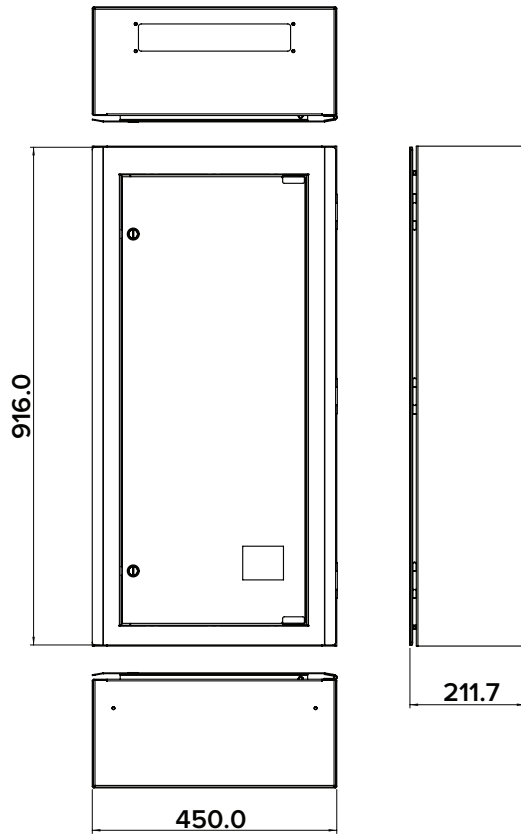
Large Enclosure
