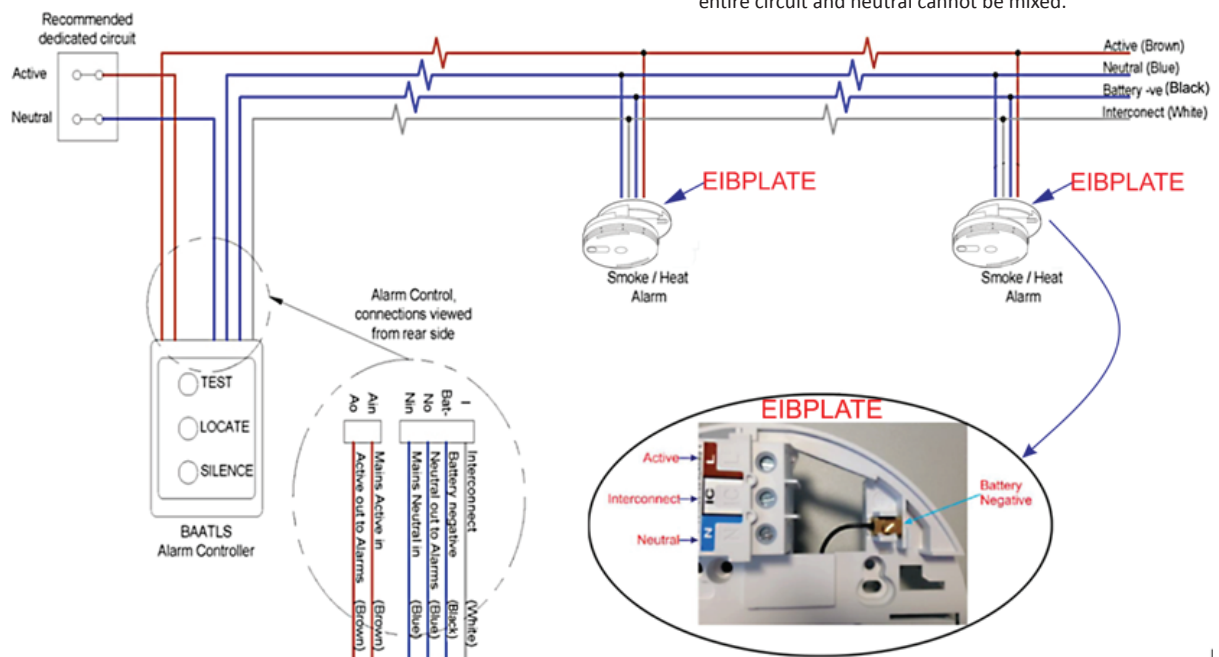
Figure 1 BAATLS Wiring Diagram
