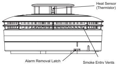
EiB660i Multi-Sensor Alarm
